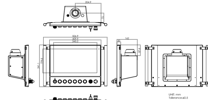
Swing Arm Top
