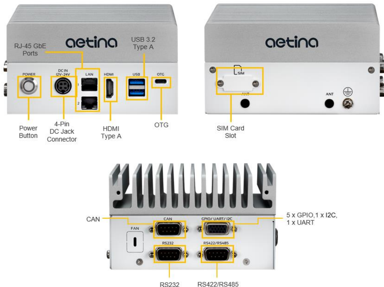
Figure 2.1 AIE-PO22/AIE-PO32/AIE-PN32/AIE-PN42 I/O Interface
