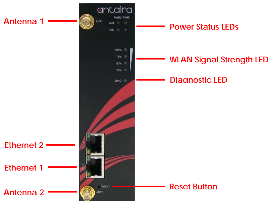
Front Panel of the APN-310N
