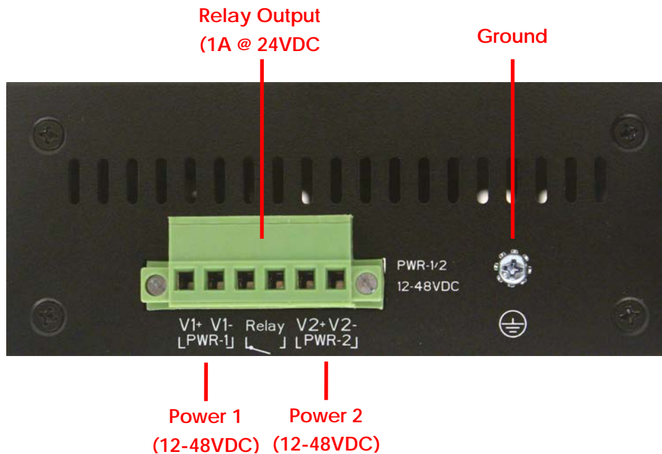
Top panel of the APN-310N
