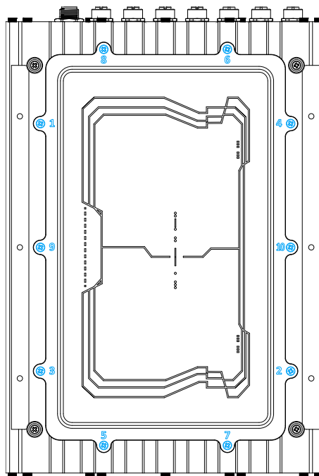
Attach the backplate, incremental screw order, and at a specified torque range (6.3 to 7.7 kgf-cm)
